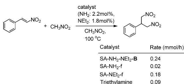
Scheme 4. The amine-catalyzed Michael reaction of 2 and 3 .
